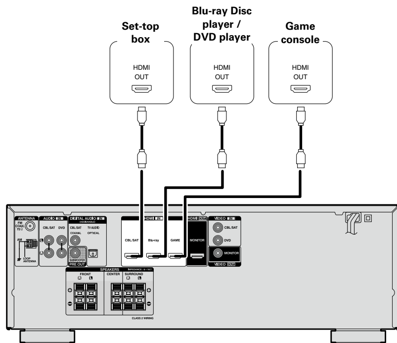
[Rear panel]
